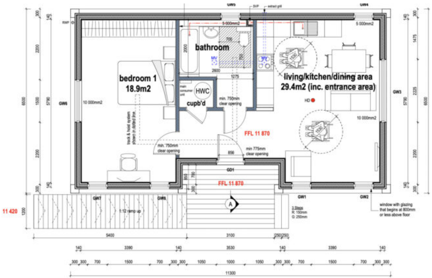
proposed around floor plan
